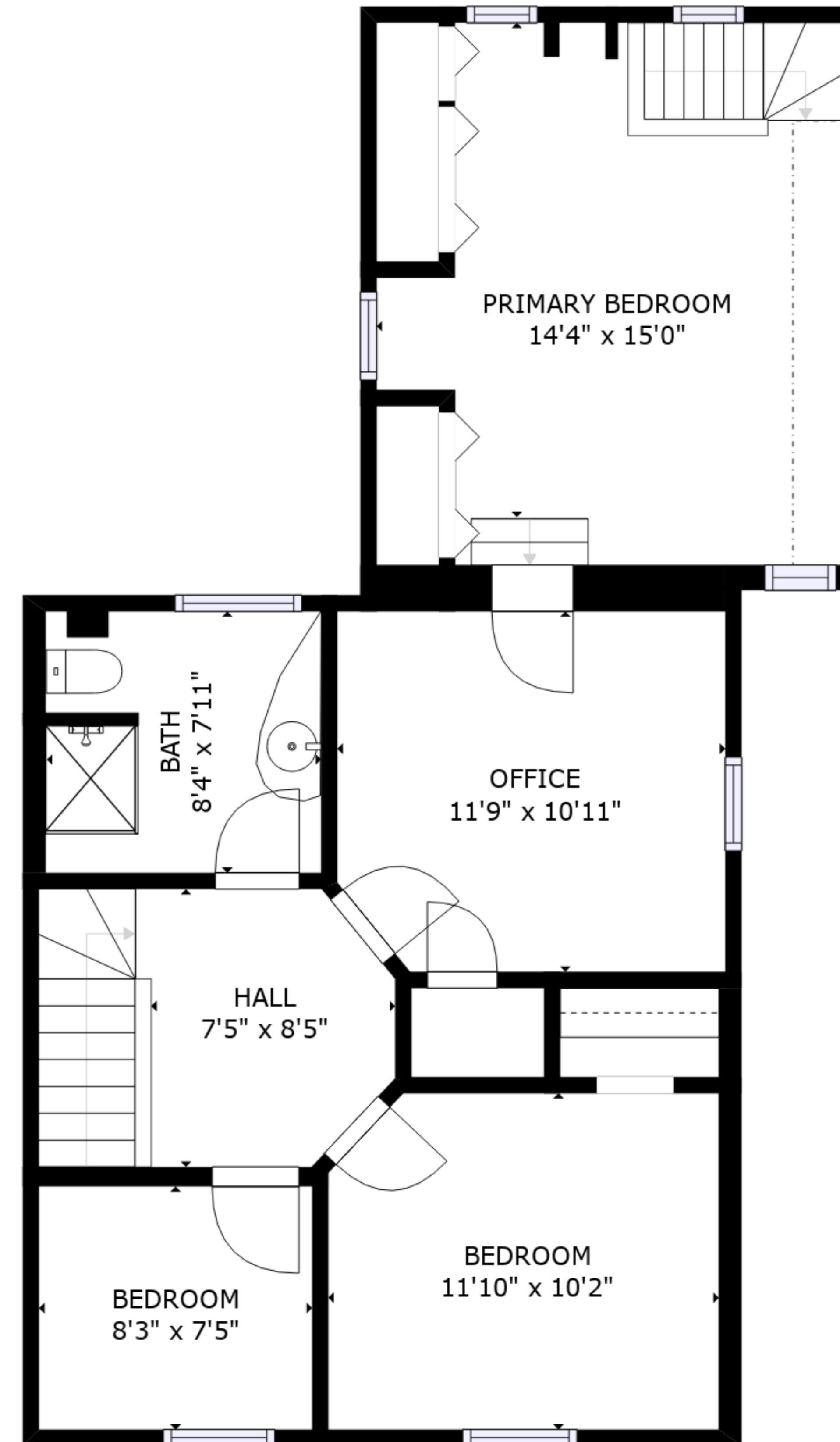
FLOOR 2
